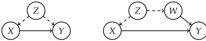
Figure 33: Two cases of unobserved confounding.
