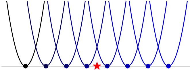
Figure 19: Plot of the different increments of \frac{1}{2n} \sum_{i=1}^n (w - y_i)^2 . The red star denotes the optimal solution.
