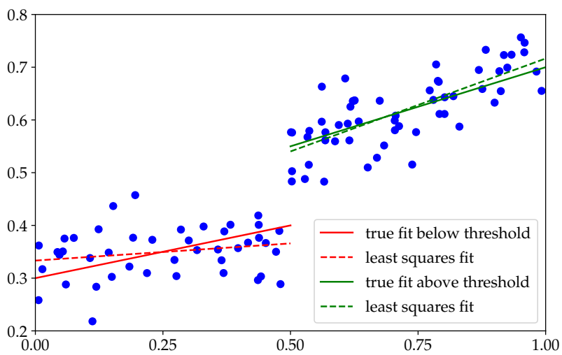
Figure 35: Illustration of an idealized regression discontinuity. Real examples are rarely this clear cut.
