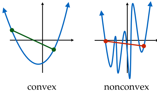
Figure 15: Convex vs nonconvex functions.
