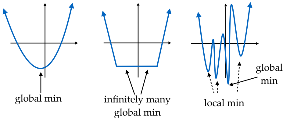
Figure 14: Examples of minima of functions. In the first illustration, there is a unique minimizer. In the second, there are an infinite number of minimizers, but all local minimizers are global minimizers. In the third example, there are many local minimizers that are not global minimizers.
