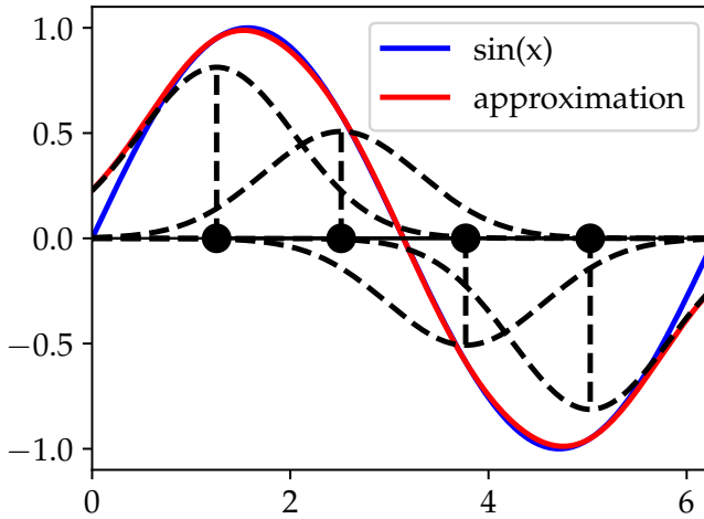
Figure 11: Radial Basis Function approximation of \sin(x) . We plot the four Gaussian bumps that sum to approximate the function.
