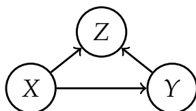
Figure 31: Example of a collider.
