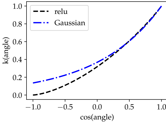
Figure 13: Comparison of the Gaussian and Arcosine Kernels. Plotting the kernel value as a function of the angle between two unit norm vectors.
