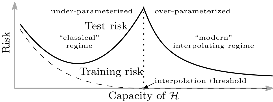
Figure 21: An extended picture with a “double descent” shape accounting for the overparameterized regime.
