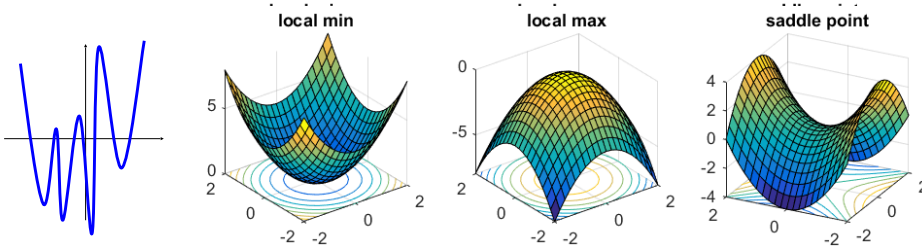
Figure 16: Examples of stationary points.
