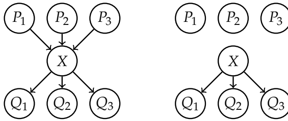
Figure 32: Graph before and after substitution.
