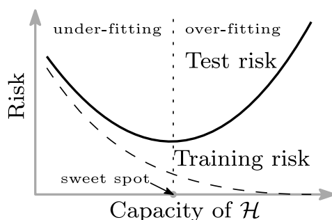
Figure 20: The so-called bias-variance trade-off represents a traditional view of generalization consistent with uniform convergence bounds
