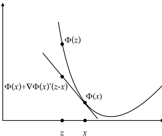
Figure 17: Tangent planes to graphs of functions are defined by the gradient. These hyperplanes always fall below the graphs of convex functions.
