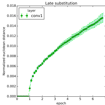
Figure 23: Parameter divergence on AlexNet trained on Imagenet. The two models differ only in a single example.
