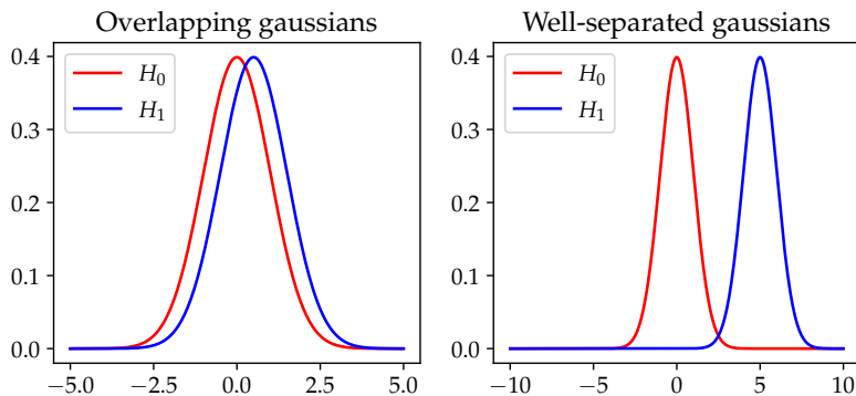
Figure 4: Illustration of shifted Gaussians
