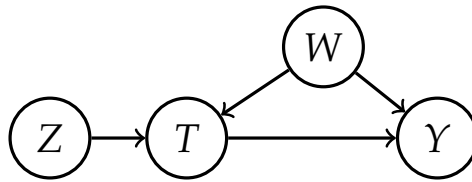
Figure 36: Typical graphical model for an instrumental variable setup
