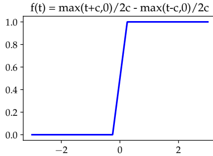
Figure 12: Creating a step function from ReLUs. Here, c=1/4 .
