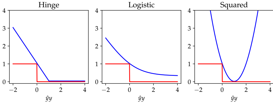
Figure 18: Example loss functions for classification. The zero-one loss is plotted in red for comparison.
