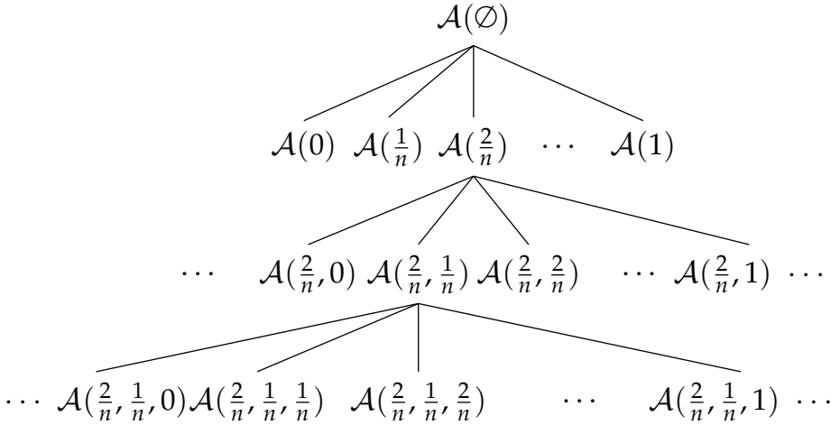
Figure 26: Constructing a tree of depth k and degree n + 1 given an adaptive analyst. Each node corresponds to the predictor the analyst chooses based on the responses seen so far.
