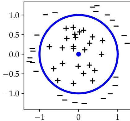
Figure 10: A cartoon classification problem for polynomial classification. Here, the blue dot denotes the center of the displayed circle.
