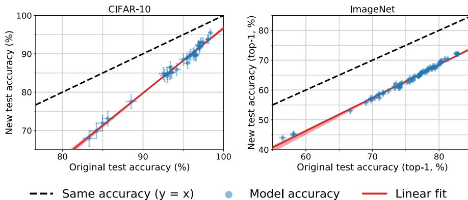
Figure 27: Model accuracy on the original test sets vs. new test sets for CIFAR-10 and ImageNet. Each data point corresponds to one model in a test bed of representative models (shown with 95% Clopper-Pearson confidence intervals). The plots reveal two main phenomena: (i) There is generally a significant drop in accuracy from the original to the new test sets. (ii) The model accuracies closely follow a linear function with slope greater than 1 (1.7 for CIFAR-10 and 1.1 for ImageNet). This means that every percentage point of progress on the original test set translates into more than one percentage point on the new test set. The two plots are drawn so that their aspect ratio is the same, i.e., the slopes of the lines are visually comparable. The narrow shaded region is a 95% confidence region for the linear fit from 100,000 bootstrap samples.
