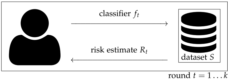
Figure 25: The adaptive analyst model. The risk estimate need not equal the empirical risk.
