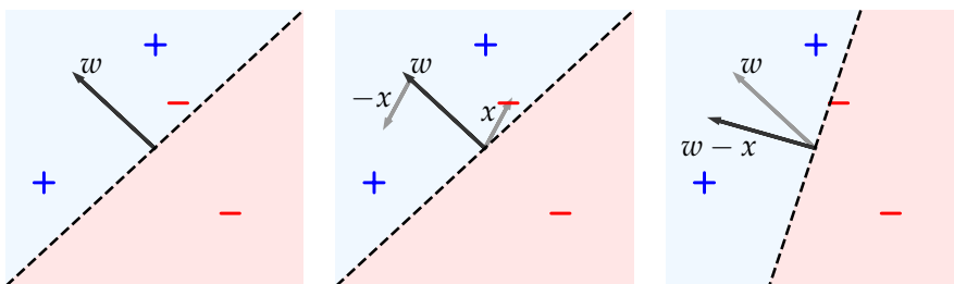
Figure 8: Illustration of the perceptron update. Left: One misclassified example x . Right: After update.
