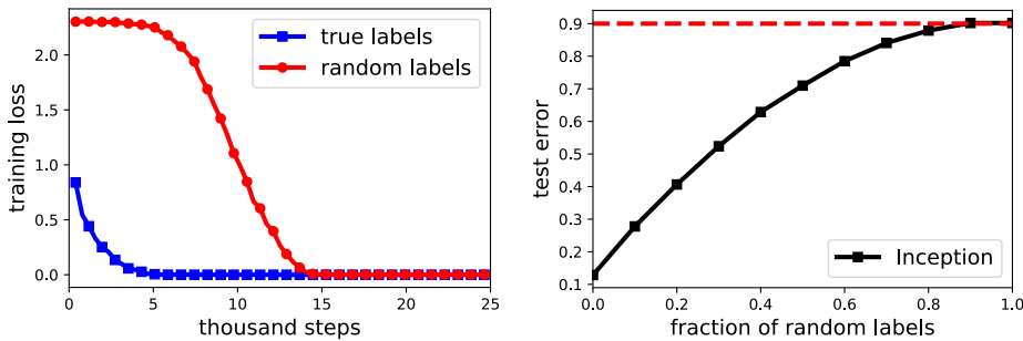
Figure 22: Randomization test on CIFAR-10. Left: How randomization affects training loss. Training still converges to zero loss even on fully randomized labels. Right: How increasing the fraction of corrupted training labels affects prediction error on the test set. At full randomization, the test error degrades to 90%, as good as guessing one of the 10 classes.
